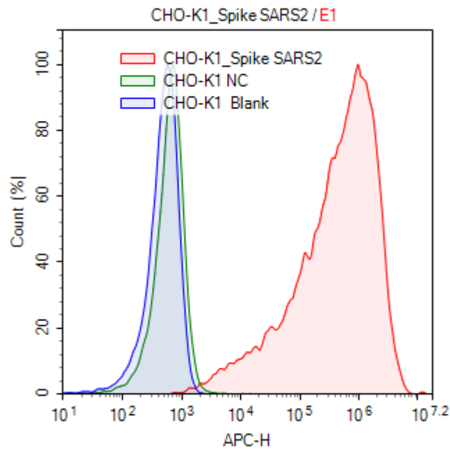
Figure 1. Flow cytometric analysis of CHO-K1/Spike_SARS2 cells after binding with ACE2 protein.
